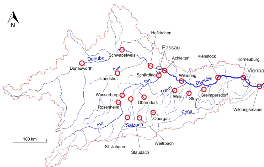
Fig. 1. Upper Danube basin upstream of Wildungsmauer. Red circles indicate stream gauges used in this paper. Black circles indicate the cities of Vienna and Passau. For catchment areas and mean elevations of the catchments see Table A1.
