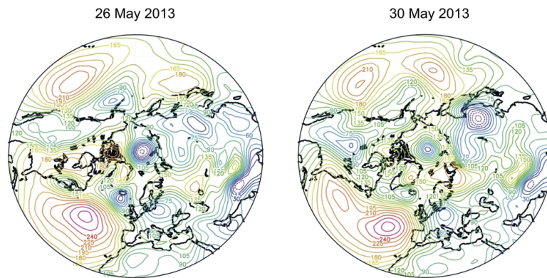
Fig. 2. Geopotential height fields (in m) at 1000 hPa of the Northern Hemisphere for latitudes above 20°. Five-day moving averages, centred on 26 May and 30 May 2013. Based on the NCEP-NCAR Reanalysis datasets (Kistler et al., 2001).
