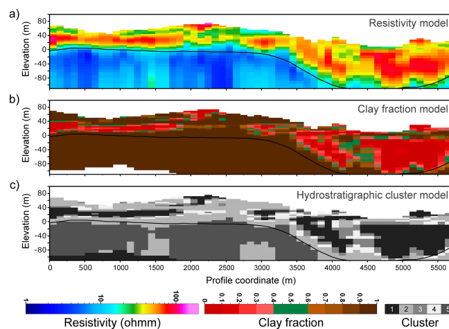
Figure 2. Northwest-southeast profiles (vertical exaggeration x5), location is marked in Fig. 3. (a) Resistivity model, (b) clay fraction model, and (c) hydrostratigraphic cluster model for the 5-cluster case.
