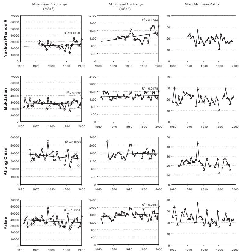
Fig. 4b. Comparisons of maximum, minimum discharge and maximum/minimum ratios at four stations (Nakhon Phanom, Mukdahan, Khong Chiam and Pakse) in the lower portion of the study area. 2319
