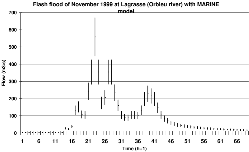
Fig. 10. Observed Flood Hydrograph at Lagrasse.
