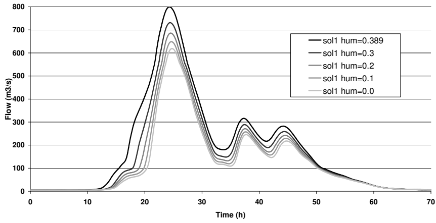
Fig. 13. Influence of the initial water content of the soil on a flash flood hydrograph with a Green and Ampt infiltration model.
