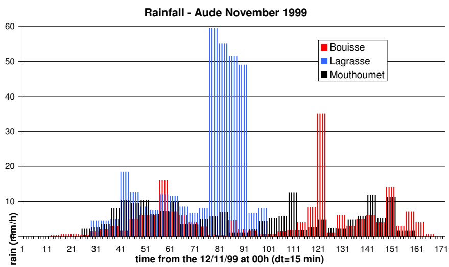
Fig. 8. Bouisse, Mouthoumet and Lagrasse pluviographs (rain in mm/h).
