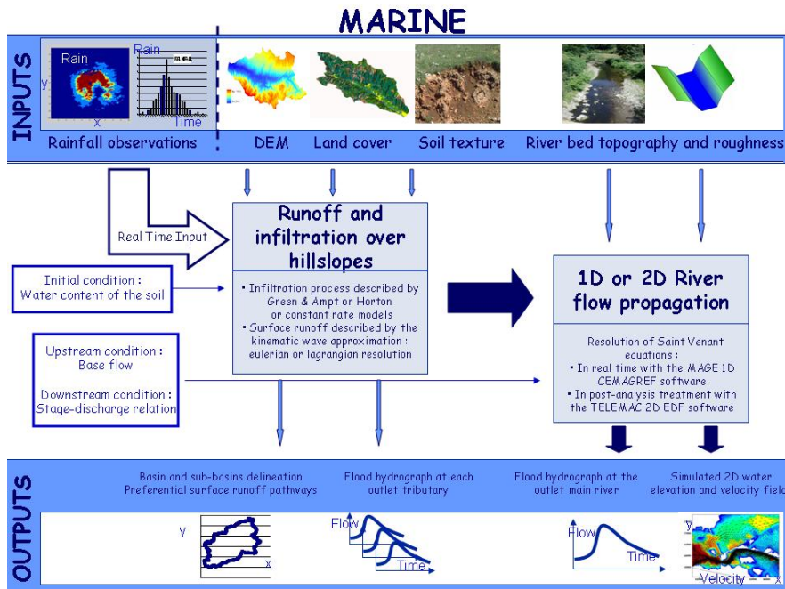
Fig. 1. General flow-chart of the MARINE hydrological model.
