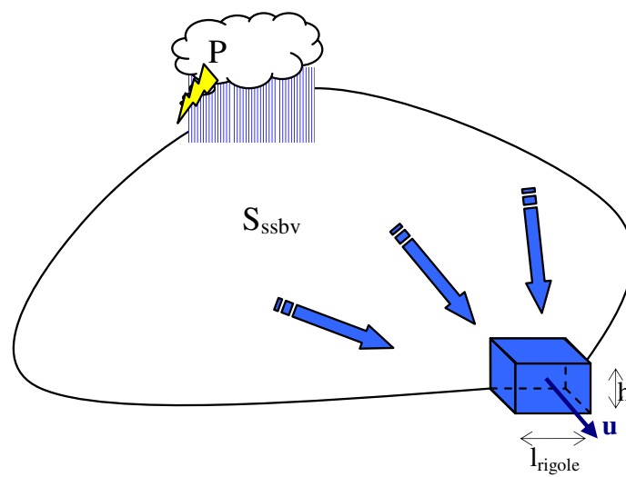
Fig. 4. Balance for the blue pixel size ( S_{ssbv} : area of the basin upstream the pixel, u : water velocity on the pixel, l_{rigole} : width of the “channel” draining water, h : water depth on the pixel).
