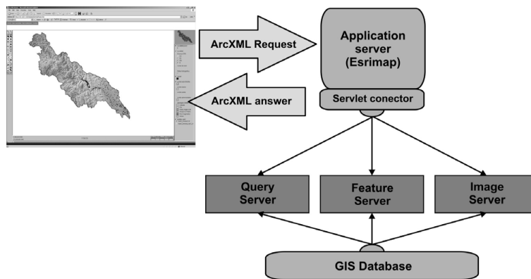
Fig. 5. ArcIMS structure.
