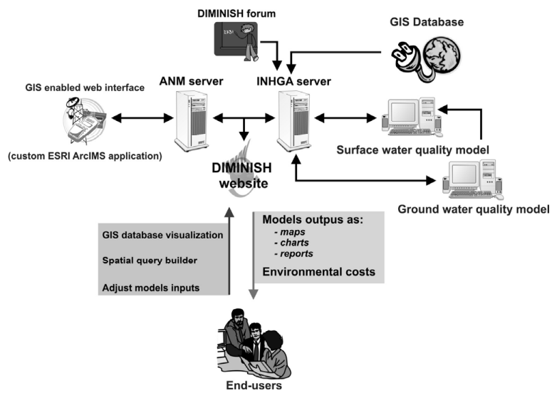
Fig. 4. DIMINISH on-line system flow-chart.
