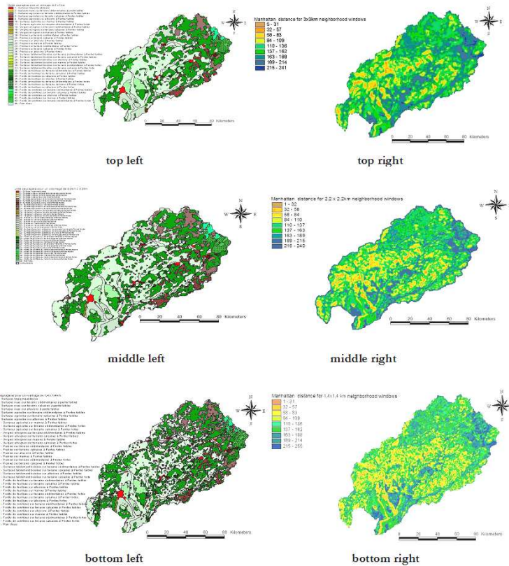
Fig. 7. Left: hydro-landscapes units and Right: distance map for three sizes of the neighbourhood window; top: 3 km, middle: 2.2 km; bottom: 1.4 km.
