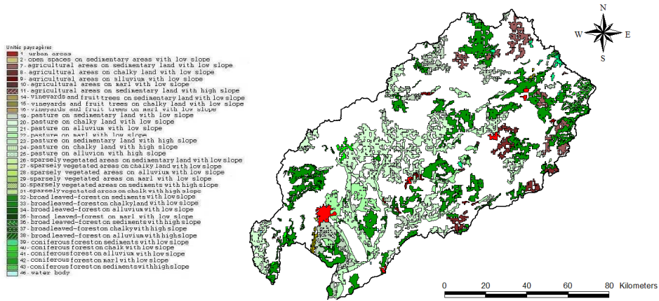
Fig. 6. Map of the reference zones.
