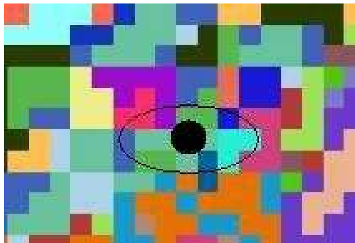
Fig. 1. Illustration of the neighbourhood windows definition.
