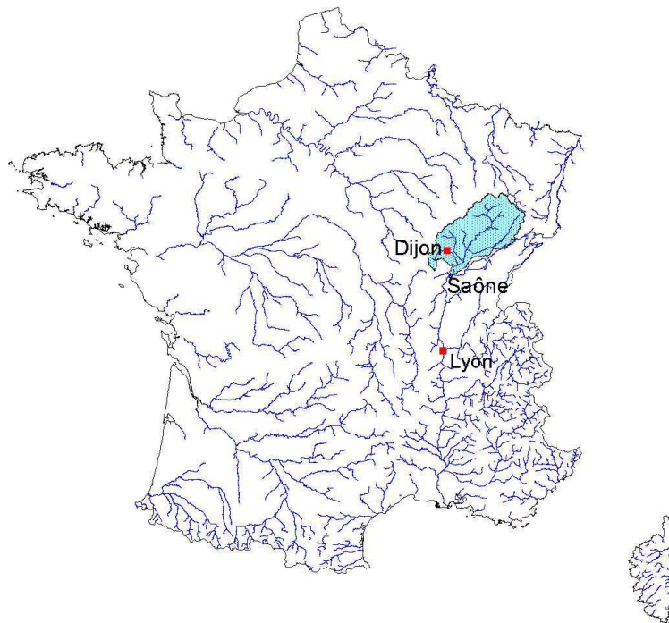
Fig. 3. Location of the upper-Saône catchment in France.
