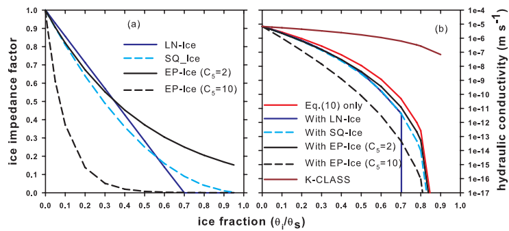
Fig. 4. (a) Parameterisations of ice impedance factor and (b) their reductions to hydraulic conductivity when applied to Eq. (10). The soil hydraulic parameters used are as in Fig. 3d.
