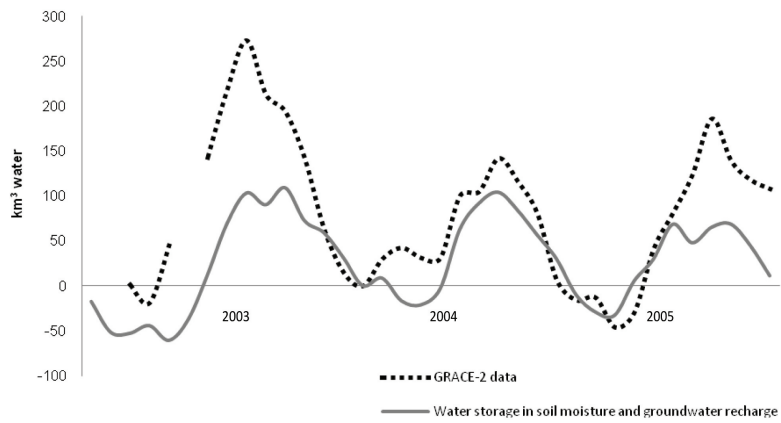
Fig. 7. Comparison of GRACE data for the Nile Basin to the total water volume stored in soil moisture and groundwater recharge. In drier years (e.g. 2004) when the volume of seasonal runoff water and surface water storage is less, the total water storage mass variation in the basin, is comprised predominantly of seasonal change in soil moisture and groundwater storage.
