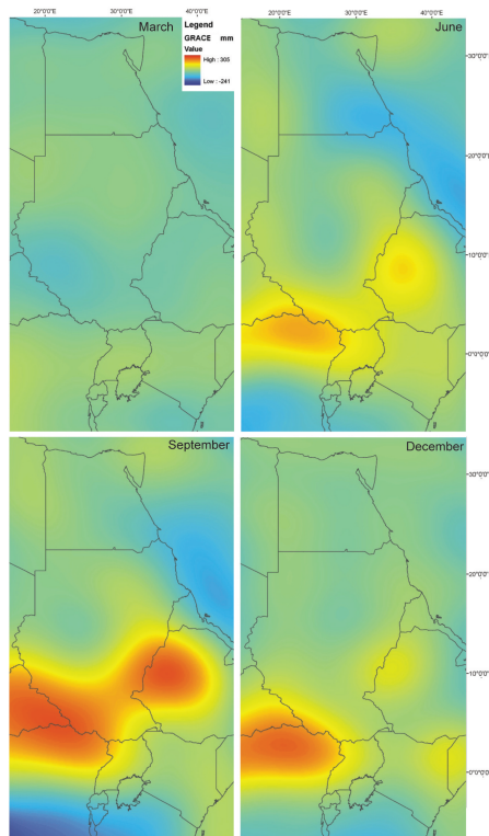
Fig. 2. GRACE data for the Nile Basin, inferred to relate to changes in terrestrial water storage mass changes. Each month of GRACE data reflects the change in total stored water mass, relative to stored water mass in March 2004 (the driest hydrological month of the modelled period).
