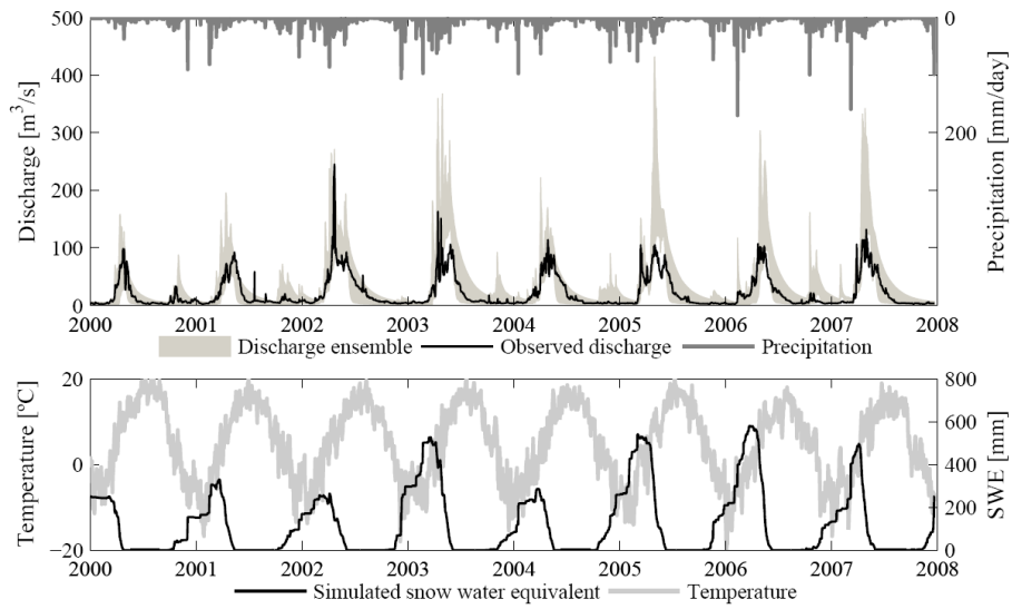
Fig. 6. Rainfall-runoff modelling results in catchment 69.
