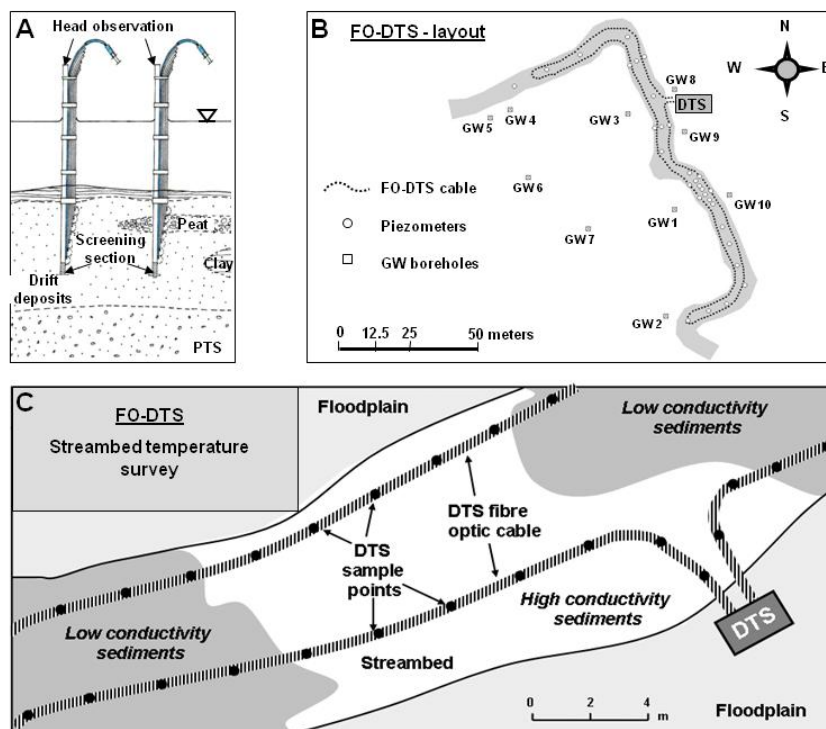
Fig. 3. Experimental installations at the River Tern with (A) streambed piezometer setup for VHG monitoring, PTS = Permo-Triassic Sandstone. (B) FO-DTS cable loop in the investigated meander bend; (C) close-up of cable layout in the streambed sediment. (The outline of the low-conductivity sediments is hypothetical.)
