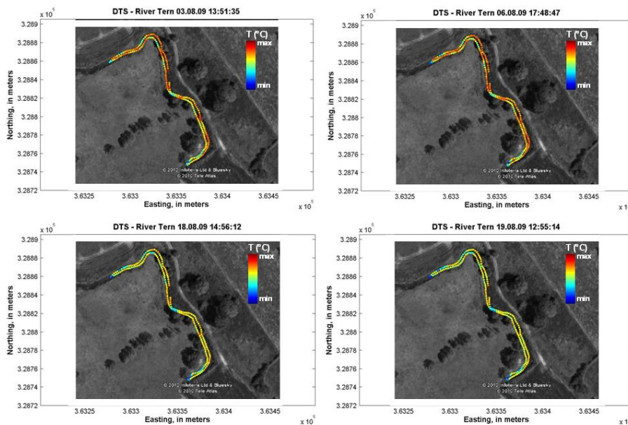
Fig. 7. Spatial patterns streambed temperature anomalies measured with FO-DTS on 4 representative sampling dates in August 2009. The colour scheme covers a range of 3 °C for all 4 maps (absolute temperatures varied slightly from one sampling date to the other).
