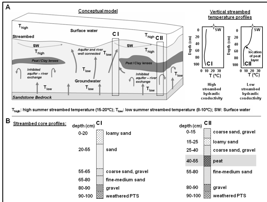
Fig. 2. (A) Conceptual model of streambed hydrofacies controlling groundwater up-welling in a typical lowland river including their effect on heat transport at the aquifer-river interface (the star indicates the temperature of the surface water). (B) Core logs of exemplary streambed cores (for sampling locations see Fig. 1).
