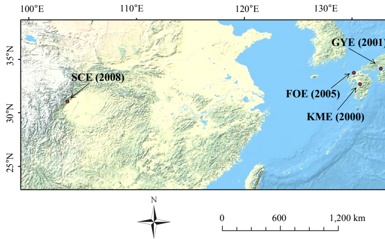
Fig. 4. Locations of the epicenters of four earthquakes that affected the groundwater levels in the Kumamoto City area. The Kumamoto Earthquake in 2000 (KME), the Geiyo Earthquake in 2001 (GYE), the Fukuoka West Offshore Earthquake in 2005 (FOE), and the Sichuan Earthquake in 2008 (SCE).
