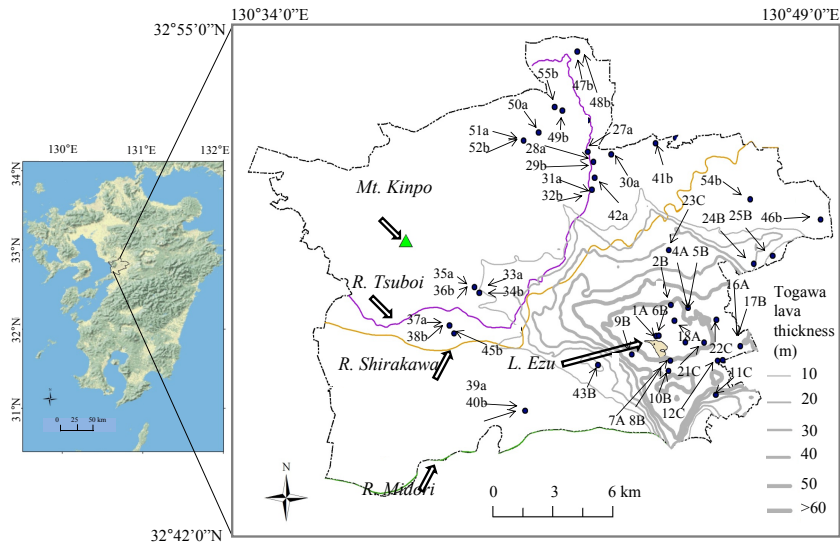
Fig. 2. Location of the study area and distribution of 54 wells used to monitor groundwater levels. The thickness of the Togawa lava is overlapped with the distribution on the basis of three-dimensional geological modeling of the study area by Koike and Matsuda (2005).
