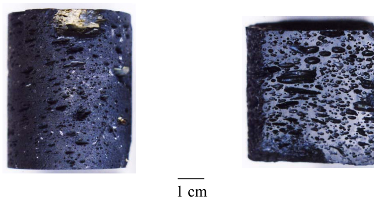
Fig. 3. Photographs of porous sections of Togawa lava (Pleistocene pyroxene andesite).
