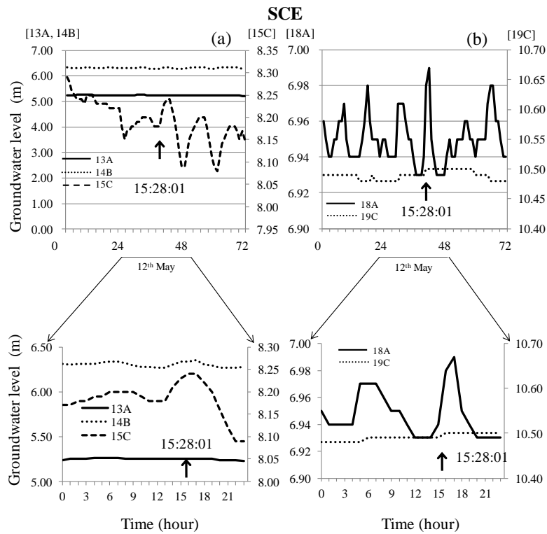
Fig. 7. Groundwater level changes over three days around the time of the SCE, the most distant earthquake, in two or three wells with the same location in the distribution of Togawa lava, but with different bottom depths (Table 2). The bottom graphs are enlargements of the day of the earthquake.
