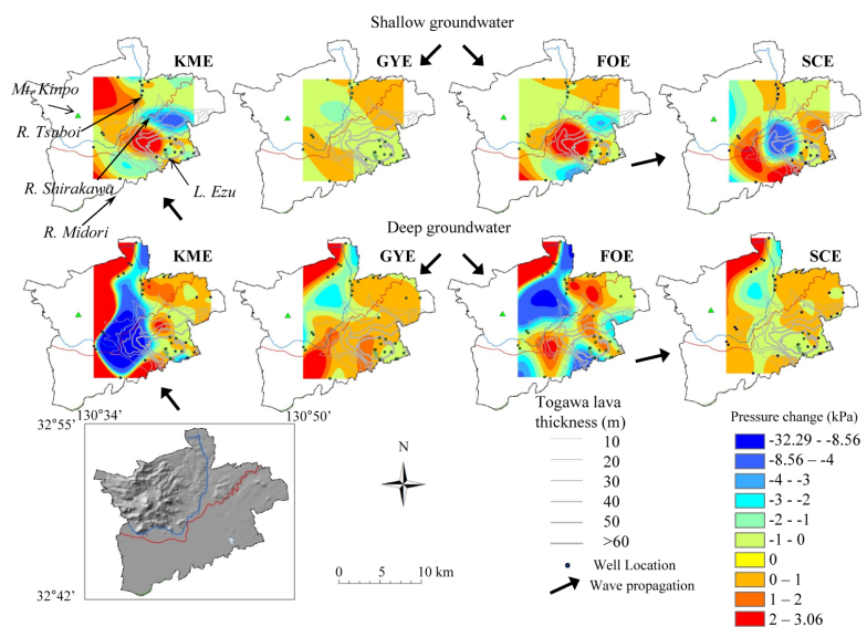
Fig. 11. Coseismic pressure change maps for the shallow and deep groundwater, calculated from Fig. 10 and using Eq. (2), in which positive and negative values mean coseismic decrease and increase of compressive stresses, respectively.
