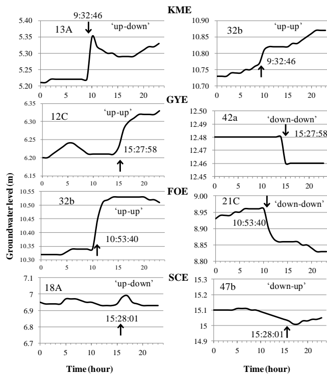
Fig. 8. Representative coseismic change patterns for groundwater levels classified in to four types, “up-down”, “up-up”, “down-up”, and “down-down”.
