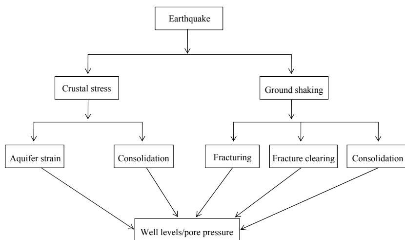
Fig. 1. Interactions between earthquakes and hydrological processes according to Montgomery and Manga (2003).
