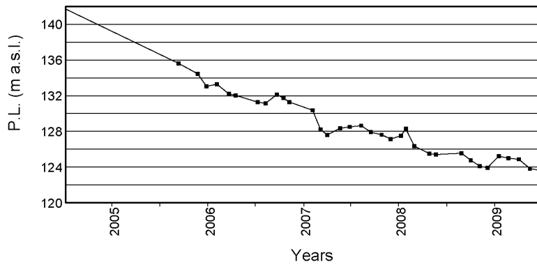
Fig. 7. Groundwater level evolution in the CHS piezometer 2.
